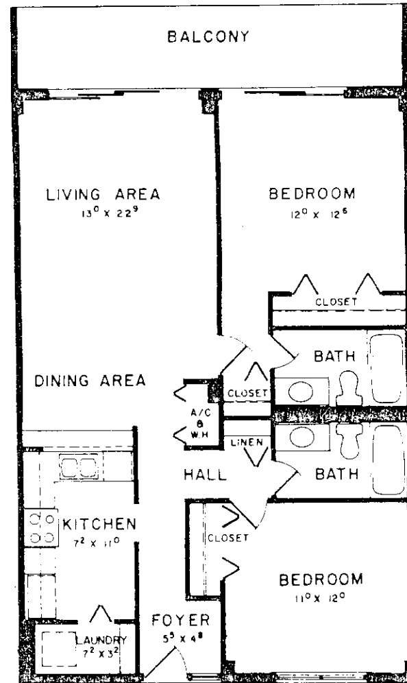
APARTMENTS 206, 306, 406, 506, 606 - AS SHOWN 212, 312, 412, 512, 612 - REVERSE
