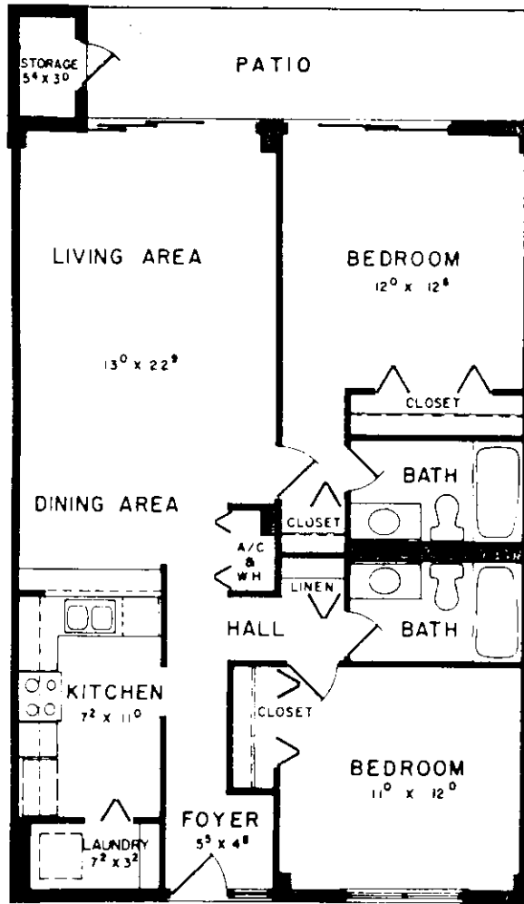
APARTMENT 103 - AS SHOWN APARTMENT 109 - REVERSE
