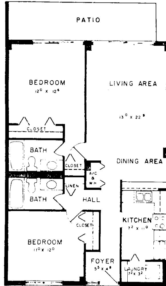
APARTMENT 104 - AS SHOWN APARTMENT 110 - REVERSE
