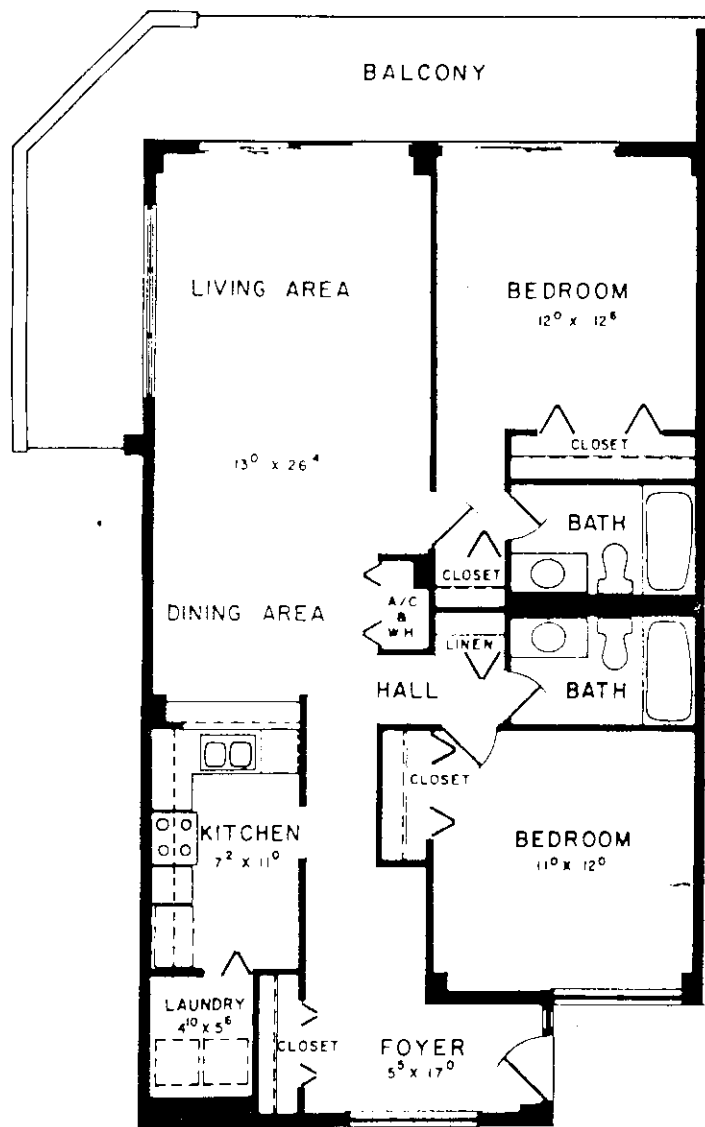
APARTMENTS 202, 302, 402, 502, 602 - AS SHOWN 208, 308, 408, 508, 608 - REVERSE
