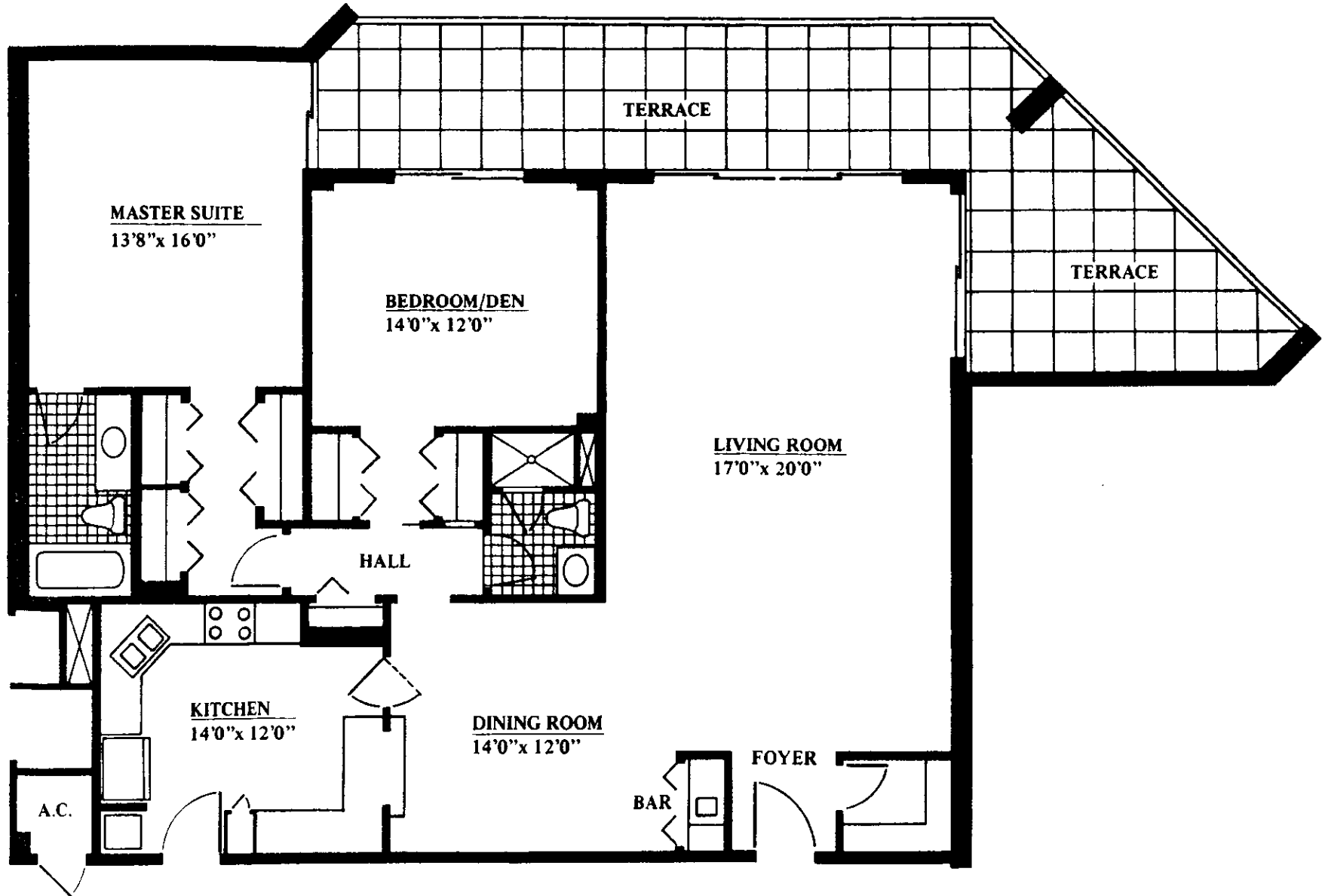
APARTMENT FLOOR PLAN "B"
