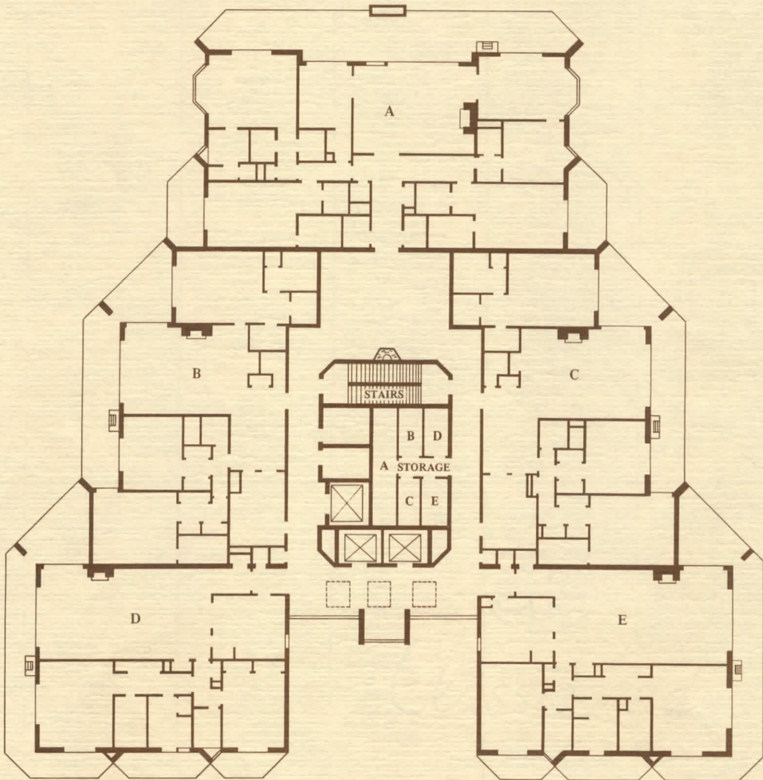
PENTHOUSE FLOOR PLAN
