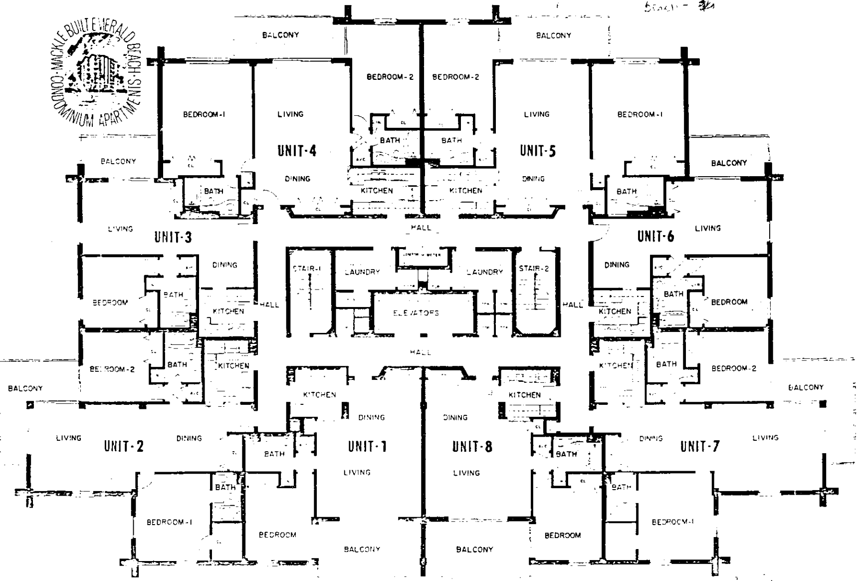
TYPICAL FLOOR PLAN (six floors - eight apartment units each floor)
